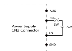
(b) Using external voltage source
