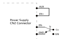
(c) ON / OFF Control by NPN transistor
